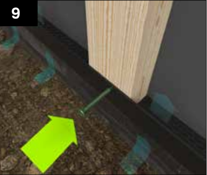
At the base of the wall attach the perforated ventilation trim to the battens. This allows for ventilation and drainage but inhibit vermin/insects. (Except for Brick Slip Rail (go to page 37), where the starter rail replaces this part)
