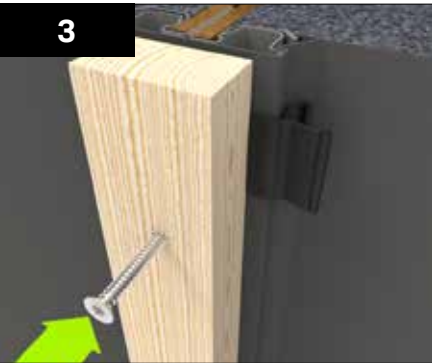
Position a 25mm batten, treated timber (optionally provided) or alternative, against the clips trapping the membrane in place. At apertures this batten is positioned inline with the opening. Secure the batten to the walling full and half clips using the winged fixing screw (provided with battens). Please Note : - Excluding flatroof, the battens will be shorter than the clip length and should be set down from the eaves level or other air flow obstructing roof elements by 12mm to allow for ventilation.
