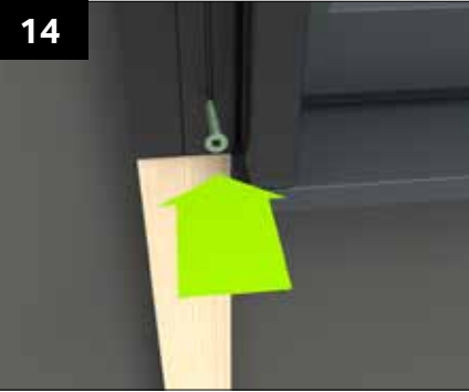
Around the perimeter of the walling openings fit the (optional) aperture trim. This will need to be cut into the cill. This is secured into the battens using GPHS.
