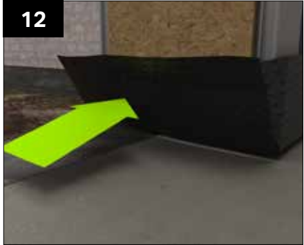
Where apertures are found at ground level fold up the excess DPC and temporarily fix in place, this can be done with tape or other method.
